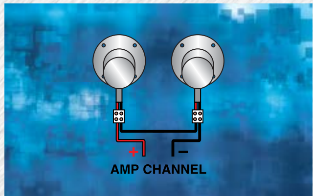
figure 4. SolidDrive's SD1 wired in series for high output installations
